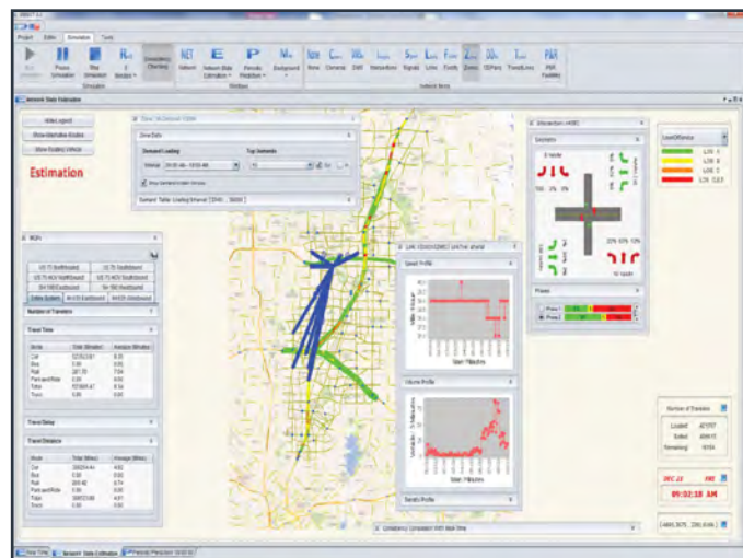
Figure 8.1 DIRECT model
